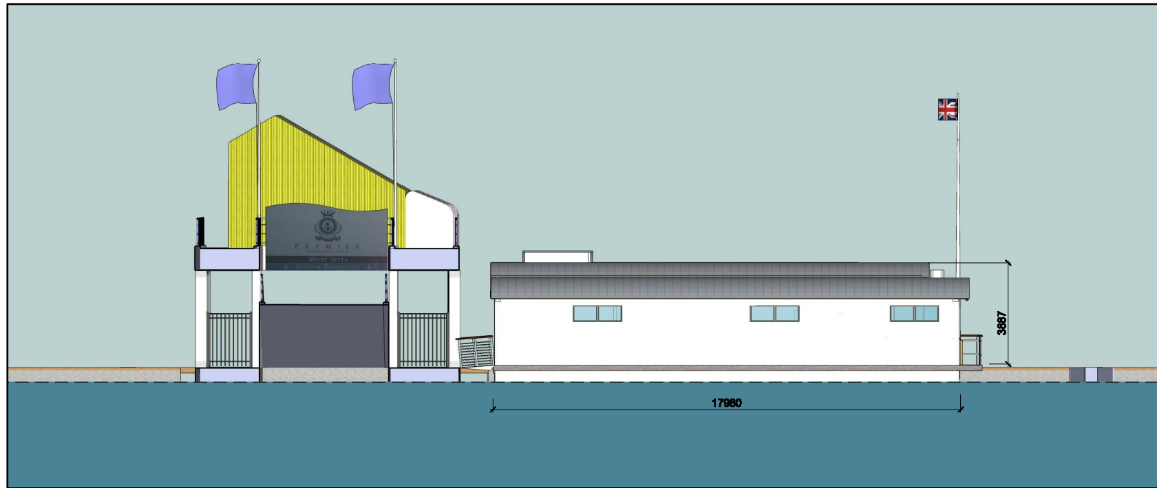
NORTHERN ELEVATION
